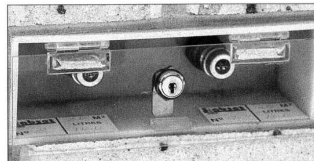
“Slab-Set” – Reticulation valves easily accessible for post-construction treatment to underslab area
