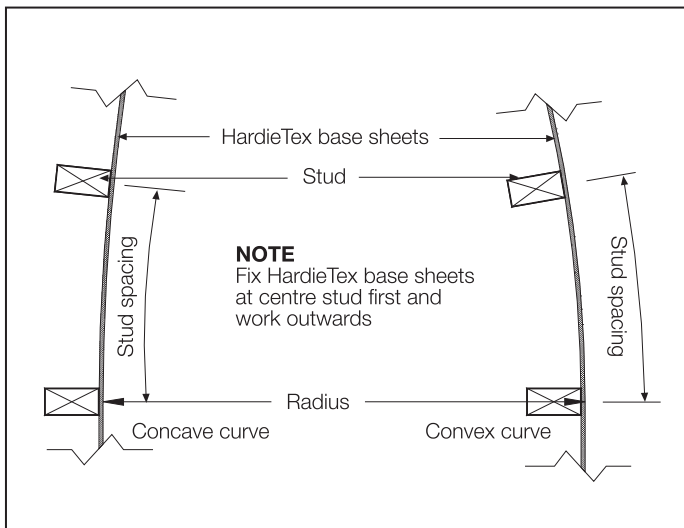
FIGURE 16 CURVED WALLS
