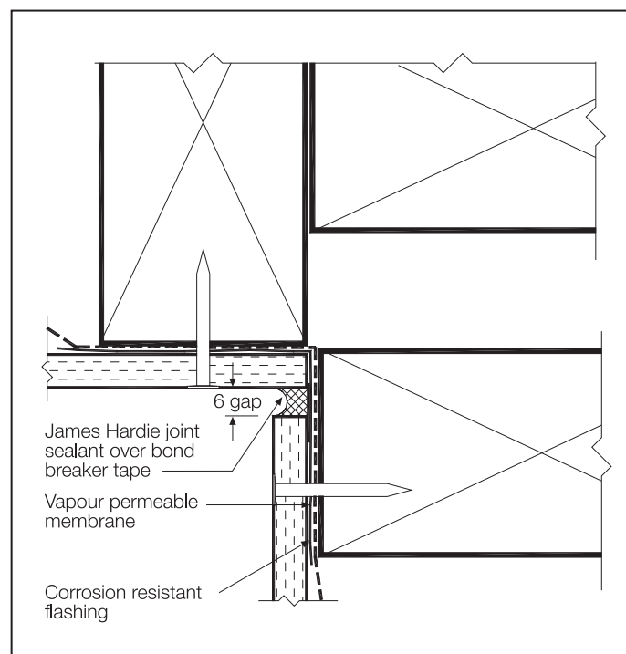
FIGURE 14 INTERNAL CORNER
