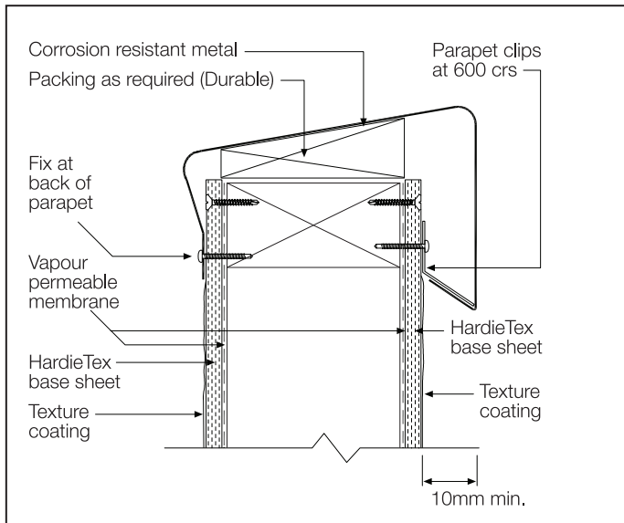
FIGURE 31 PARAPET CAPPING
