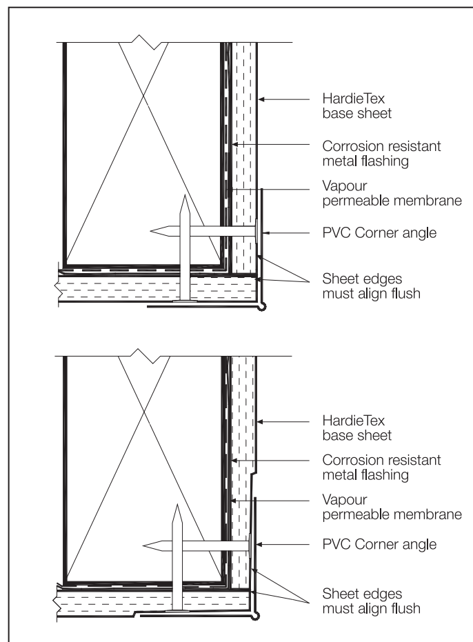
FIGURE 13 EXTERNAL CORNER OPTION 1 AND 2
