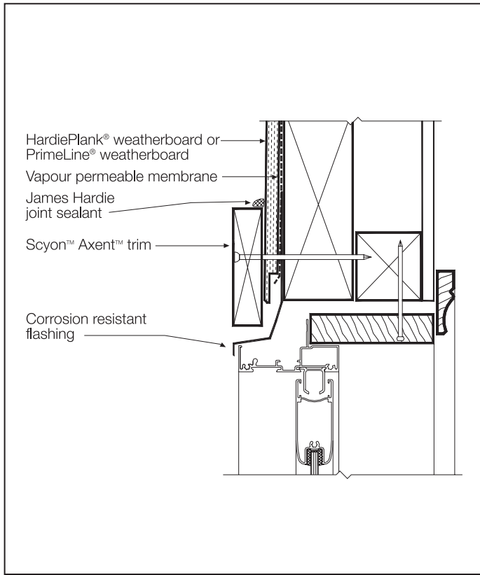
FIGURE 34 WINDOW HEAD DETAIL
