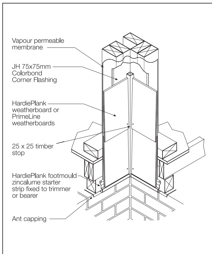
FIGURE 30 INTERNAL CORNER OPTION 2
