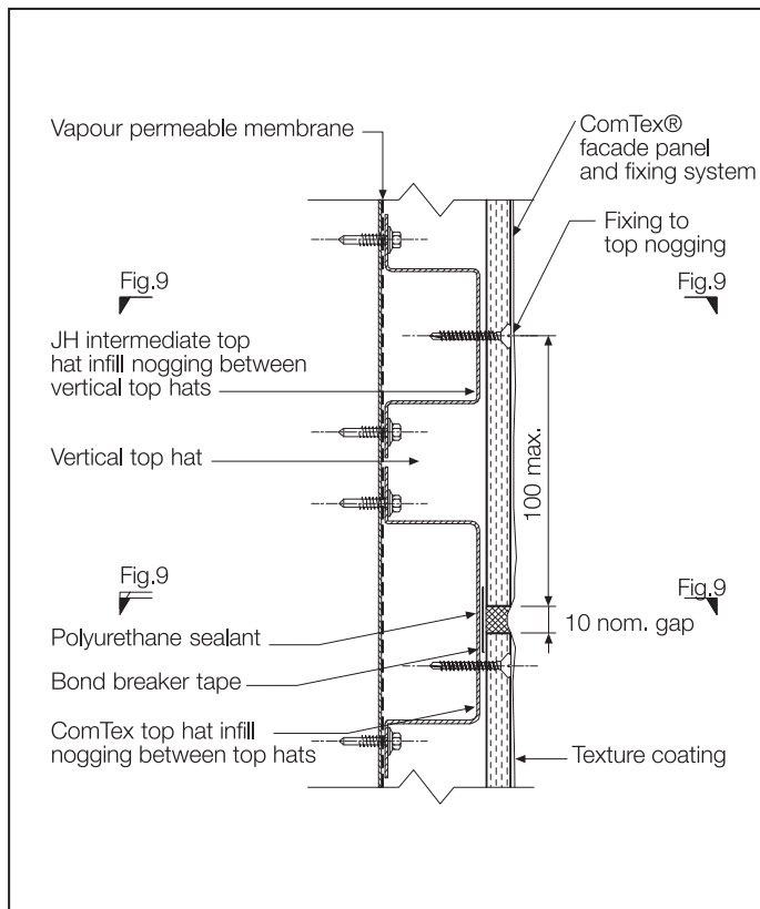
FIGURE 8 HORIZONTAL CONTROL JOINT
