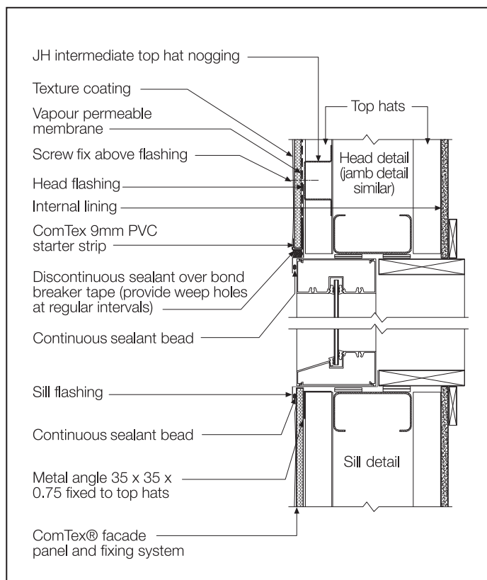
FIGURE 24 SHOP FRONT WINDOW
