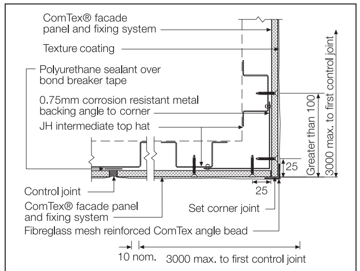
FIGURE 17 EXTERNAL CORNER
