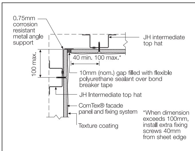
FIGURE 19 INTERNAL CORNER
