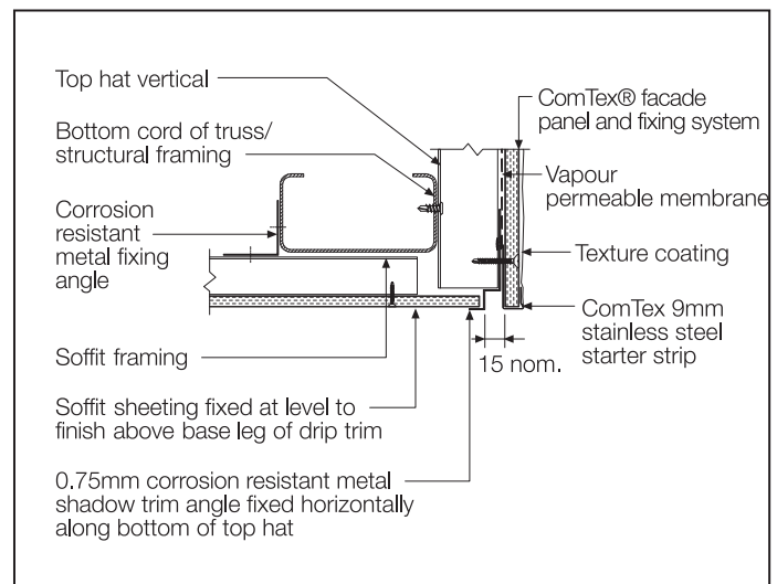
FIGURE 22 FASCIA/SOFFT JUNCTION - SHADOW DRIP GROOVE TRIM
