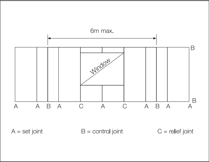
FIGURE 5 SET, CONTROL, RELIEF JOINT PANEL LAYOUT
