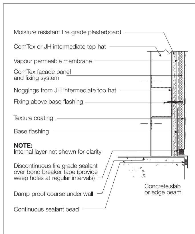
FIGURE 27 FIRE RATED COMTEX FACADE PANEL AND FIXING SYSTEM BASE DETAIL
