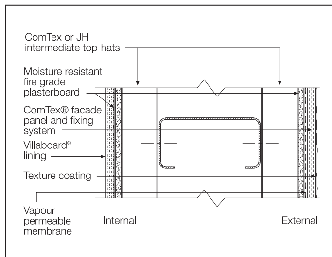
FIGURE 26 FIRE RATED COMTEX FACADE PANEL AND FIXING SYSTEM
