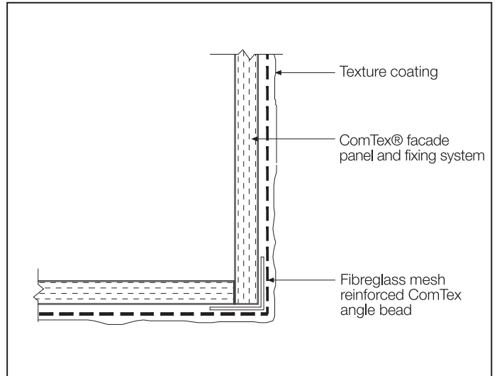
FIGURE 15 PREFERRED SET EXTERNAL CORNER
