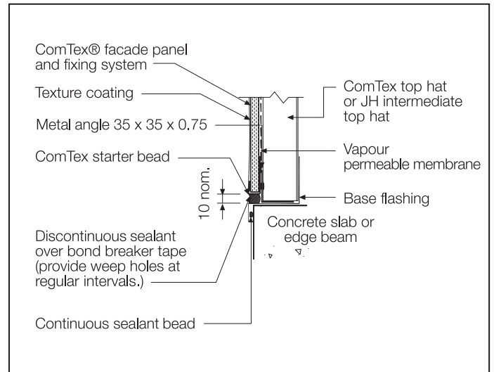
FIGURE 21 BASE DETAIL ALTERNATIVE 2
