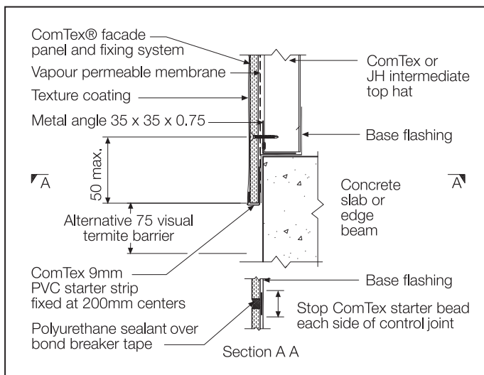
FIGURE 20 BASE DETAIL ALTERNATIVE 1
