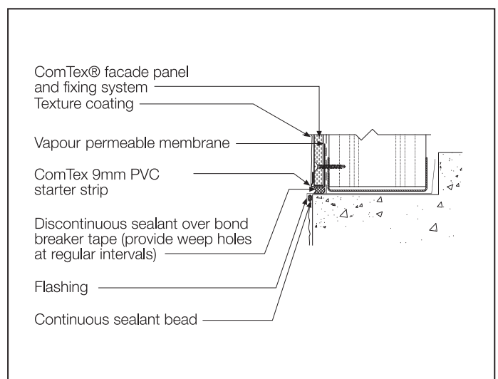
FIGURE 38 BASE DETAIL 2
