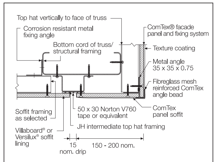
FIGURE 23 FASCIA/SOFFT JUNCTION - ALTERNATIVE SET CORNER
