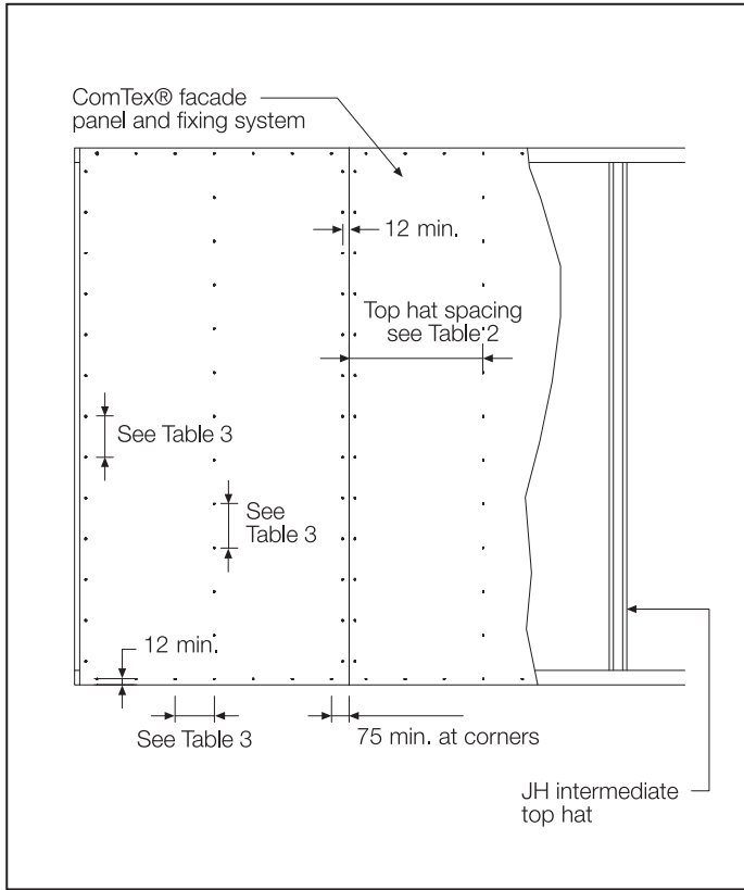
FIGURE 13 VERTICAL FACADE PANEL FIXING
