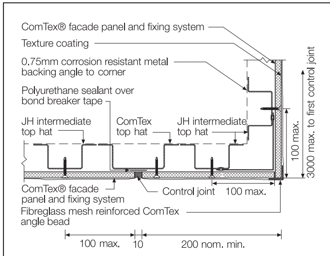
FIGURE 18 ALTERNATIVE EXTERNAL CORNER
