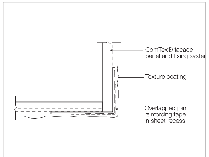
FIGURE 16 ALTERNATIVE SET EXTERNAL CORNER
