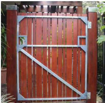
STEP 8. Re-hang your finished gate & attach your latch, lock or catch.
